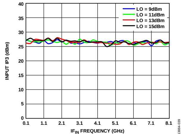
Figure 39. Input IP3 vs. IF_{IN} Frequency at Various LO Power Levels, T_A = 25^\circ\text{C}
