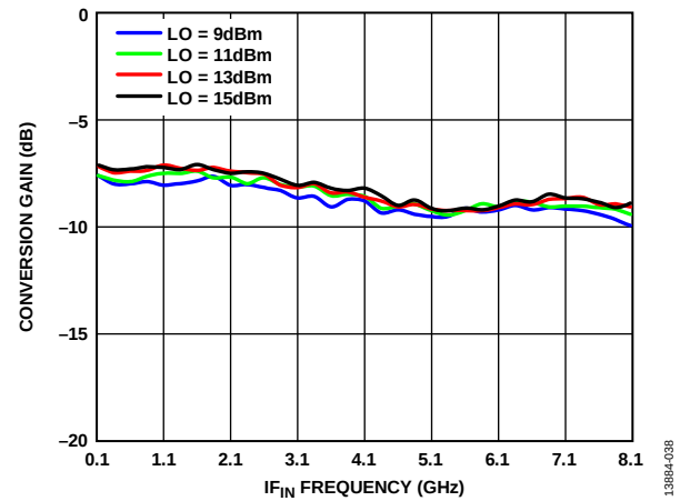
Figure 38. Conversion Gain vs. IF_{IN} Frequency at Various LO Power Levels, T_A = 25^\circ\text{C}
