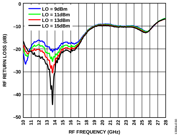
Figure 30. RF Return Loss vs. RF Frequency at Various LO Powers, T_A = 25^\circ\text{C}
