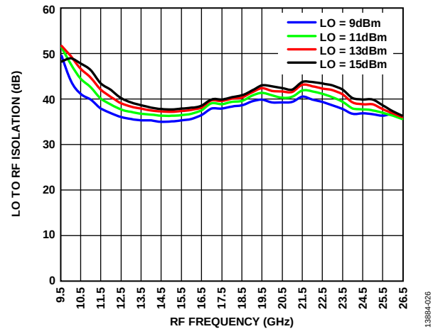
Figure 26. LO to RF Isolation vs. RF Frequency at Various LO Power Levels, T_A = 25^\circ\text{C}
