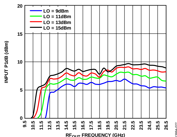
Figure 22. Input P1dB vs. RF_{OUT} Frequency at Various LO Power Levels, T_A = 25^\circ\text{C}
