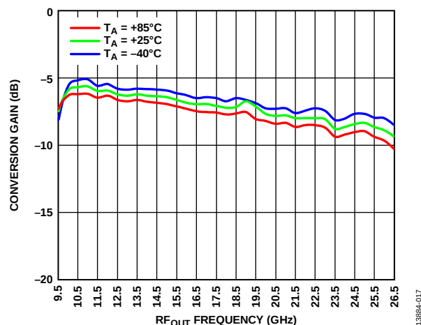
Figure 17. Conversion Gain vs. RF Output ( RF_{OUT} ) Frequency at Various Temperatures, LO = 13 dBm
