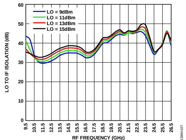
Figure 27. LO to IF Isolation vs. RF Frequency at Various LO Power Levels, T_A = 25^\circ\text{C}
