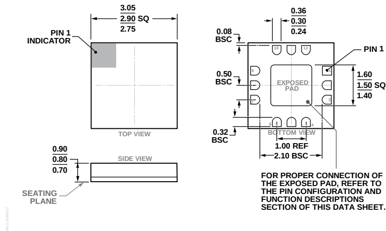
Figure 42. 12-Terminal Ceramic Leadless Chip Carrier (LCC) (E-12-4)
