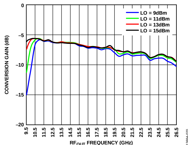
Figure 20. Conversion Gain vs. RF_{OUT} Frequency at Various LO Power Levels, T_A = 25^\circ\text{C}
