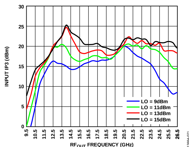
Figure 21. Input IP3 vs. RF_{OUT} Frequency at Various LO Power Levels, T_A = 25^\circ\text{C}
