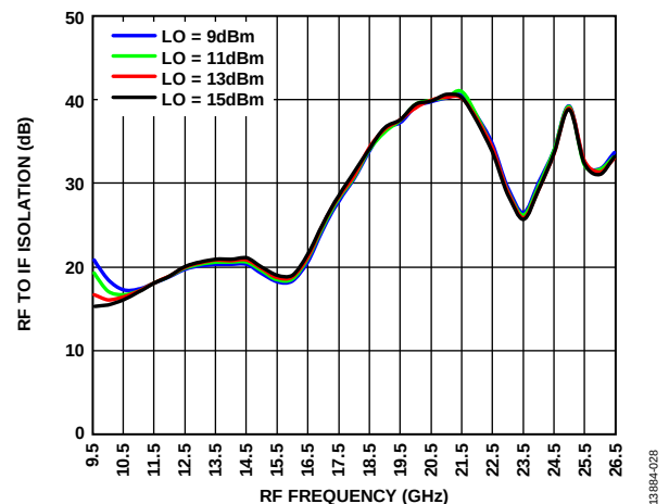
Figure 28. RF to IF Isolation vs. RF Frequency at Various LO Power Levels, LO = 17 GHz, T_A = 25^\circ\text{C}
